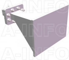
LB-159-15-C-SFSPO Standard Gain Horn Antenna 4.9-7.05GHz 15dB Gain SMA Female
