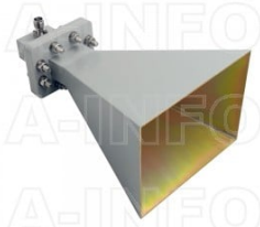
LB-159-15-C-TF Standard Gain Horn Antenna 4.9-7.05GHz 15dB Gain TNC Female
