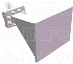
LB-159-15-C-7SPO Standard Gain Horn Antenna 4.9-7.05GHz 15dB Gain 7mm
